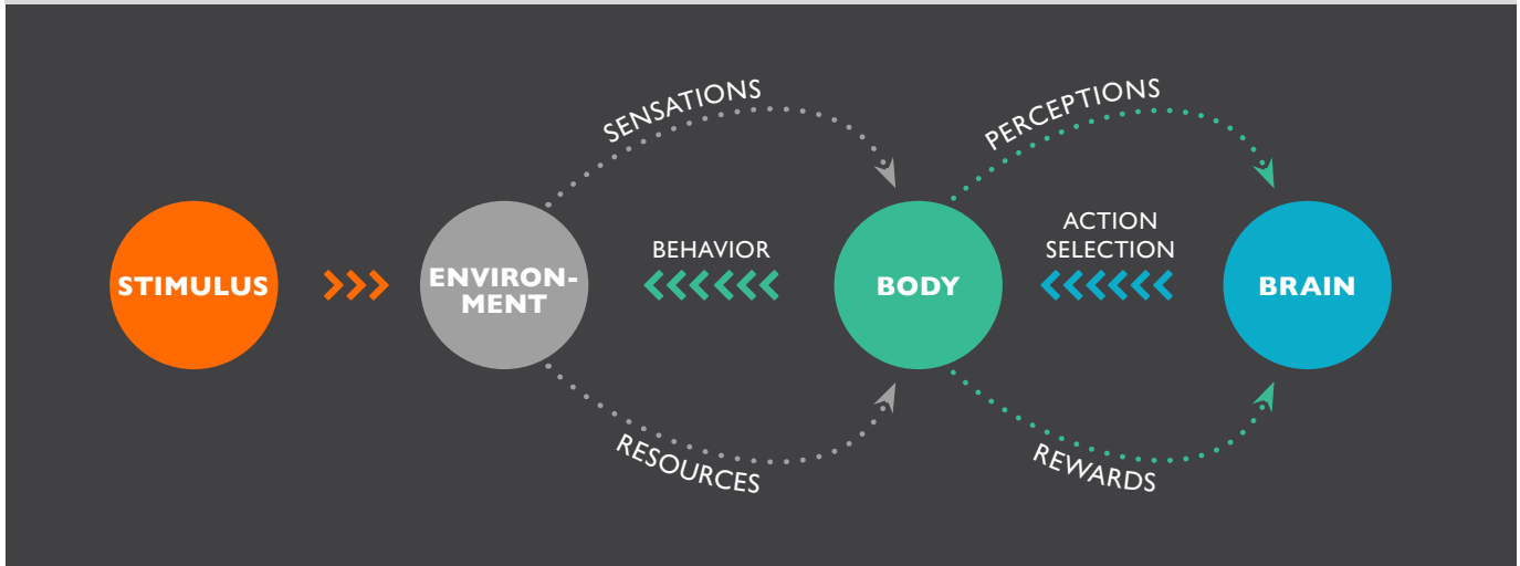
FIGURE 2: Reinforcement Learning
